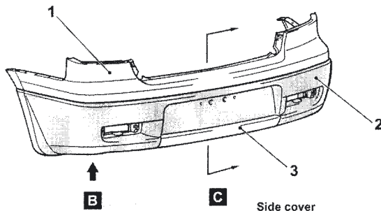
Rear bumper
